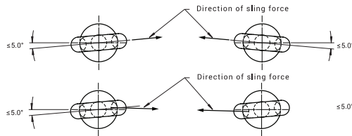
Figure 2 Alignment of eyes when using 2 leg slings
