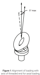
Figure 1 Alignment of loading with axis of threaded end for axial loading
