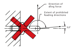
Figure 4 Angular limits of lateral loading perpendicular to the plane of the eye
